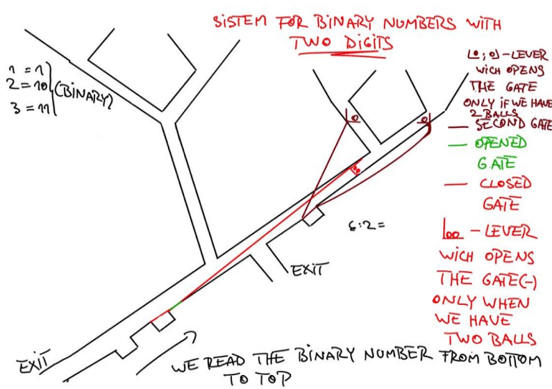
Figure 10: "Two-digit binary numbers system"
